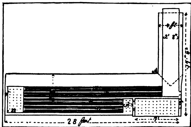
FIG. 182.—MARINE BOILER.
